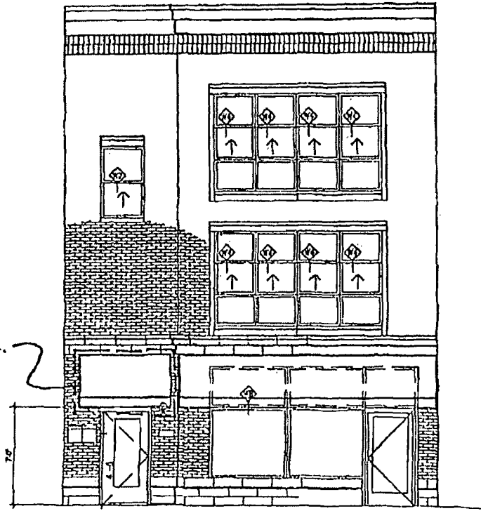
FRONT ELEVATION SCALE: 1/8\"/>
