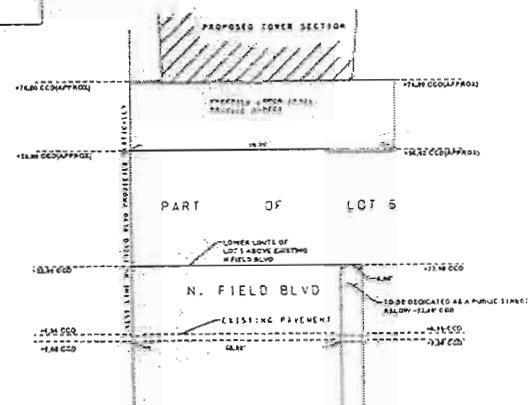
SECTION "A" LOOKING NORTH
