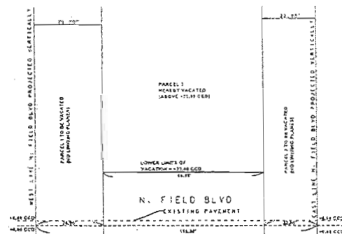
SECTION "B" LOOKING NORTH
