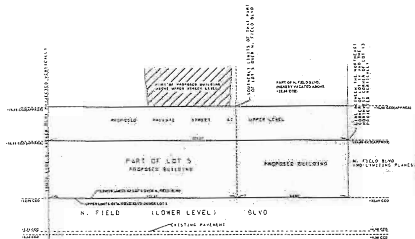
SECTION "C" LOOKING EAST
