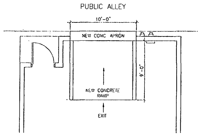
2 PARTIAL FLOOR PLAN
