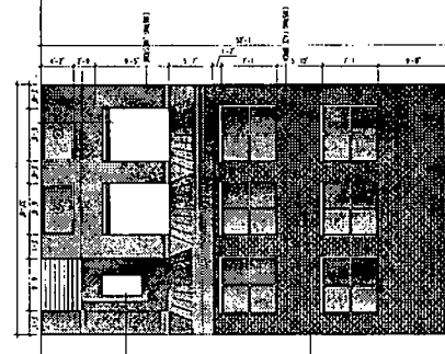
NORTH ELEVATION
