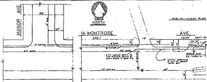
LOCATION-PLAN SCALE 1"=30 FT.
