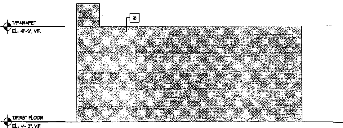
2 EXISTING PARKING LOT ELEVATION SCALE: 1/16" = 1'-0"
