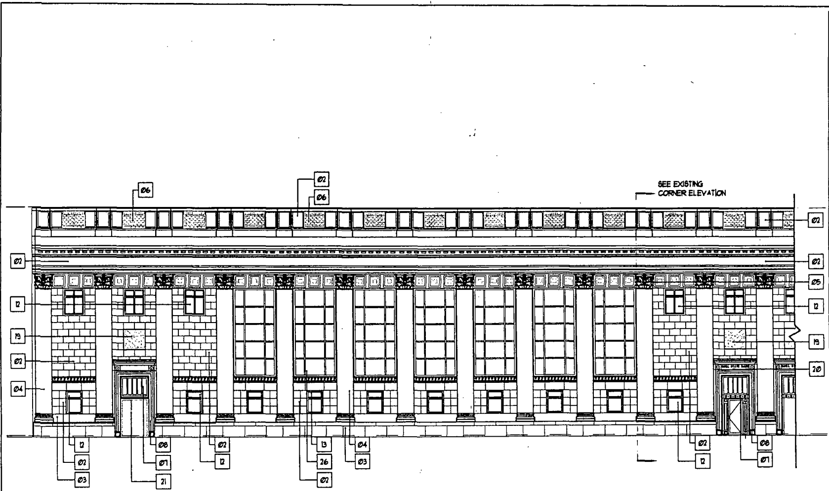
1 EXISTING SOUTHWEST ELEVATION - MILWAUKEE AVE SCALE: 3/32" = 1'-0"
