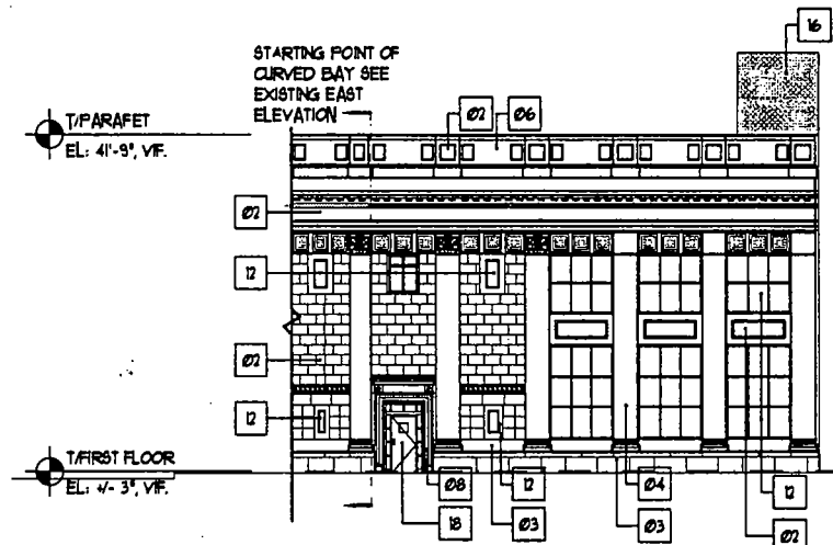
3 EXISTING ALLEY ELEVATION SCALE: 1/16" = 1'-0"
