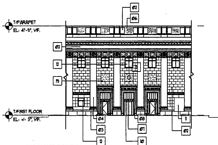
1 EXISTING CORNER ELEVATION SCALE: 1/16" = 1'-0"
